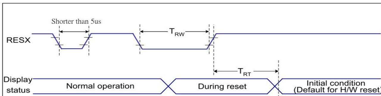
Reset Timing Characteristics IOVCC=1.65~1.95v Ta=25°C
